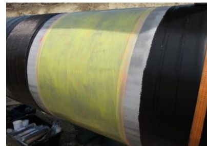
The prepared section of pipe is ready for the fiber wrap.
